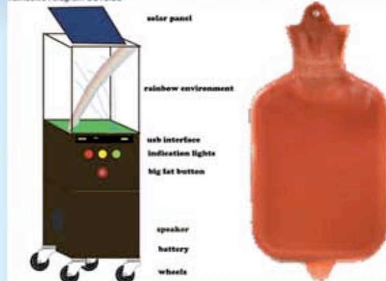
Rainbows : diagram OUTSIDE
